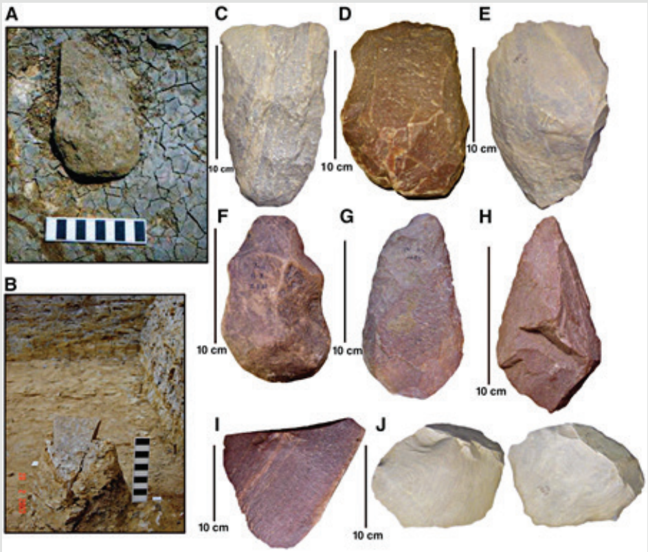
Acheulian artefacts from excavations at Attirampakkam (after Pappu et al. 2011).
