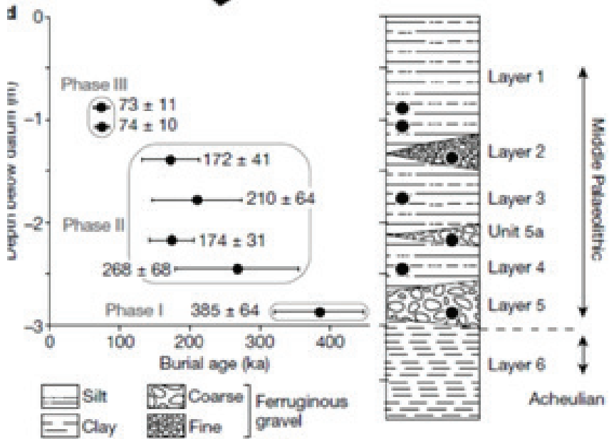
Geochronology of the Middle Palaeolithic layer at Attirampakkam (after Akhilesh et al. 2018)
